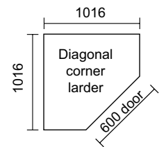
1016mm Diagonal Corner Larder Unit
