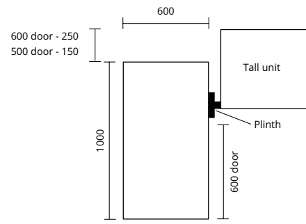
1000 Blind Corner Larder to Larder
