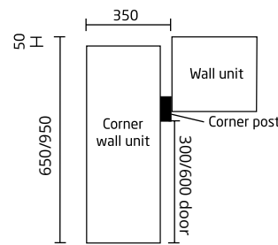
600/900mm Conventional Corner Wall Unit
