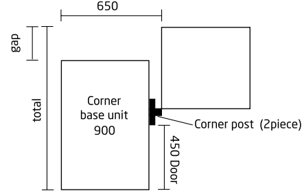
900mm Conventional Corner Base Unit
