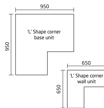
'L' Shape Corner Units Note:- Walls must be square to accommodate L shaped units.
