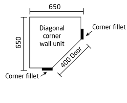
650mm Diagonal Wall Unit
