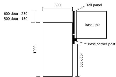
1000 Blind Corner Larder to Base Unit
